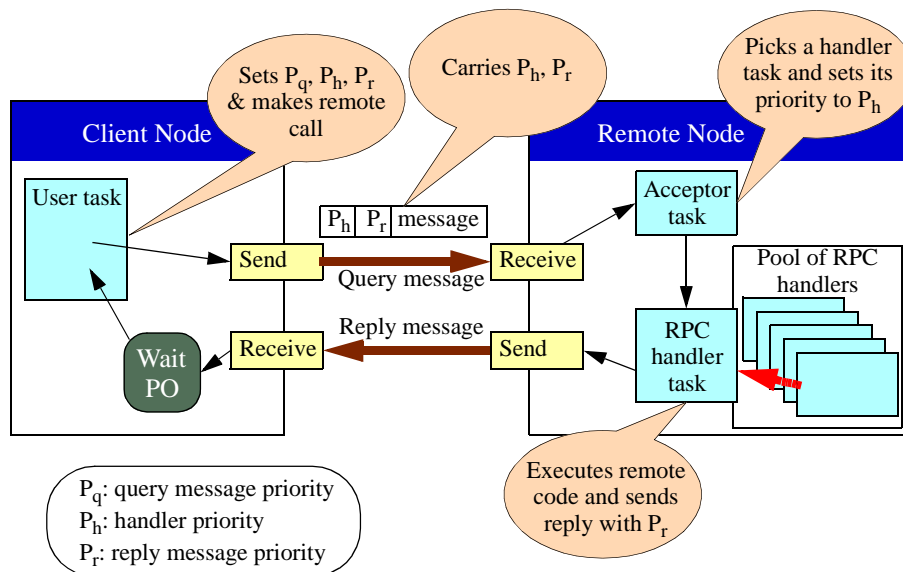
Fig. 2. Handling priorities in RT-GLADE
